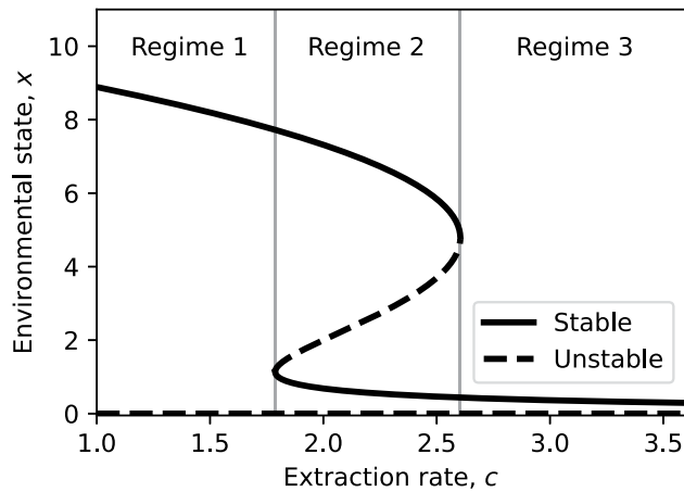
Fig. 2. For low and high extraction rates, the system has only one stable equilibrium. For intermediate extraction rates, bistability occurs and the potential for flickering dynamics arises. We use this distinction to classify our system into three distinct dynamical regimes. In regime 1, only the high environmental state is stable, regime 2 exhibits bistability and potentially flickering dynamics, and only the low environmental state is stable in regime 3. For any extraction rate, actual dynamics of the environment will fluctuate about their equilibria due to stochasticity.
